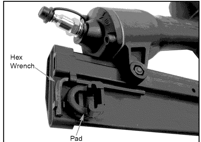
Figure 8 - Storing Contact Trip Pad and Wrench
