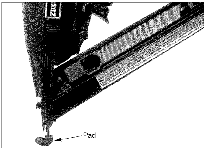
Figure 7 - Contact Trip Pad
