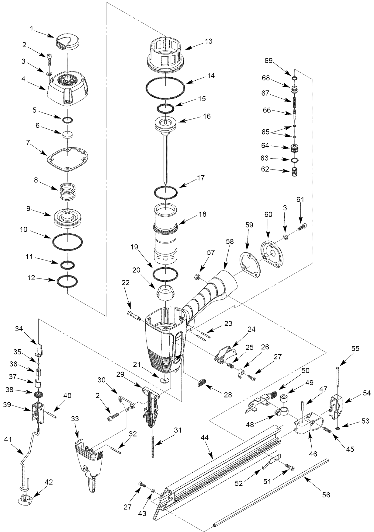
Figure 12 - Replacement Parts Illustration For Finish Nailer
